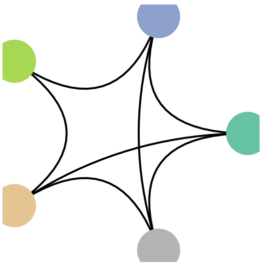
Static network
