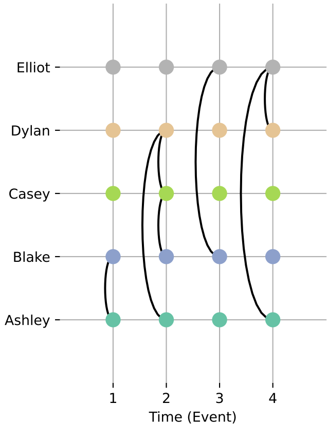
Temporal network
